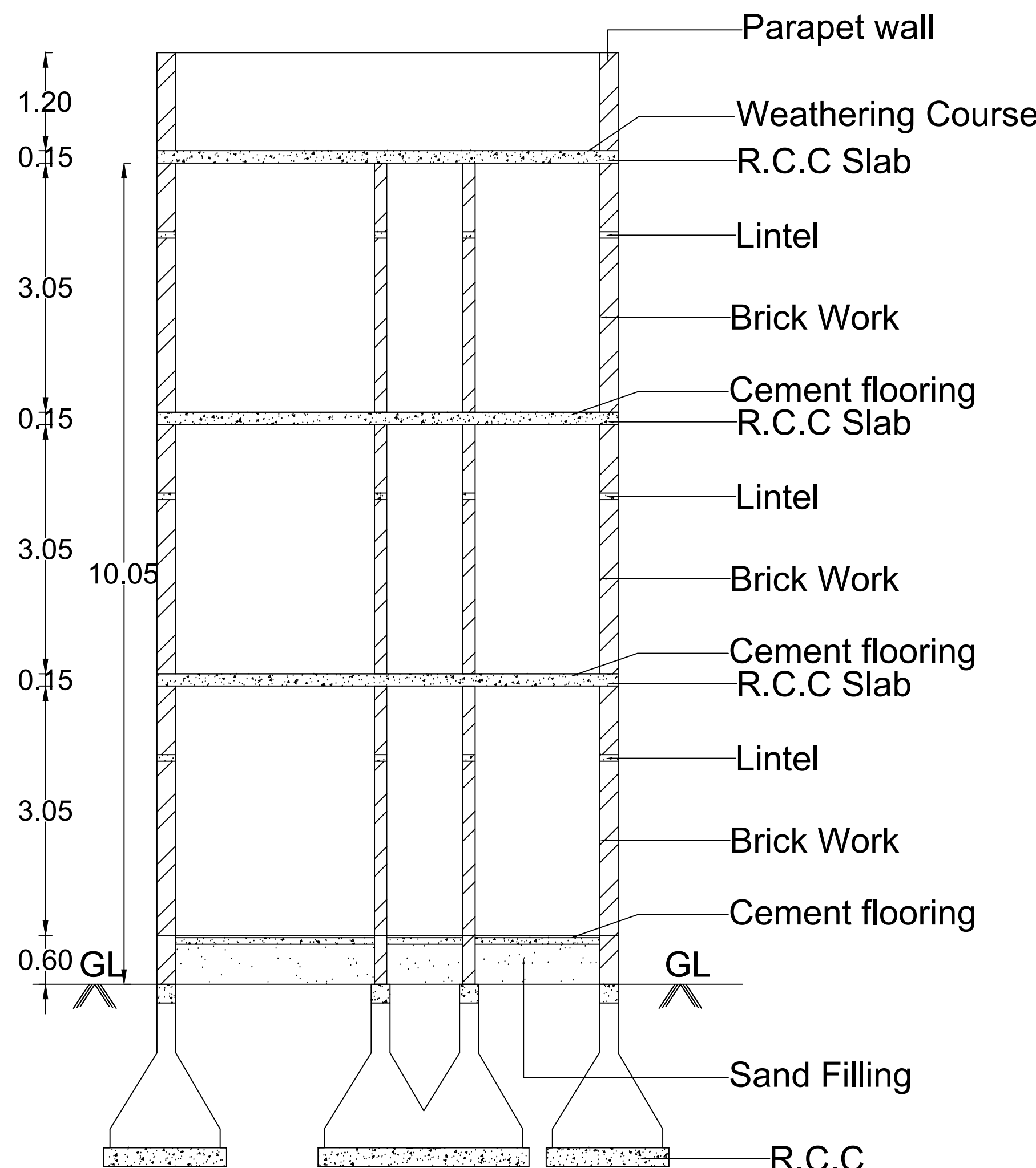
SECTION ON 'AB'
