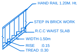
STAIR DETAIL
