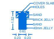
SECTION OF RAIN WATER COLLECTION TANK
