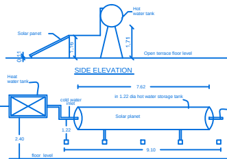
SOLAR WATER HEATER PLANT
