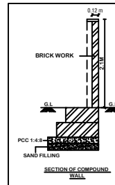
SECTION OF COMPOUND WALL
