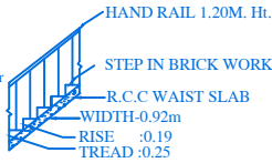
STAIR DETAIL
