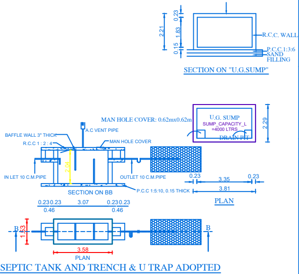
SEPTIC TANK AND TRENCH & U TRAP ADOPTED
