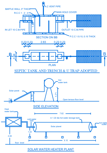
SOLAR WATER HEATER PLANT
