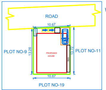
LOCATION PLAN Scale 1:400
