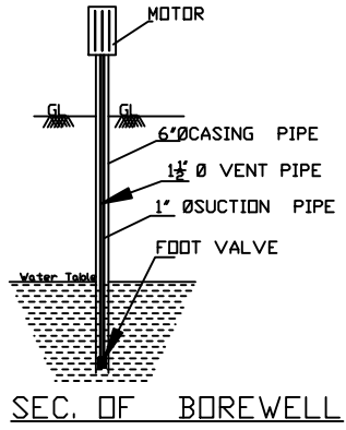
SCALE:- 1"=4'-0"
