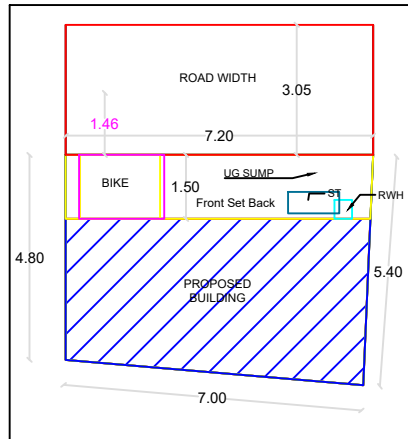
RESIDUARY PLOT SKETCH, SUPER IMPOSED (SITE PLAN)
