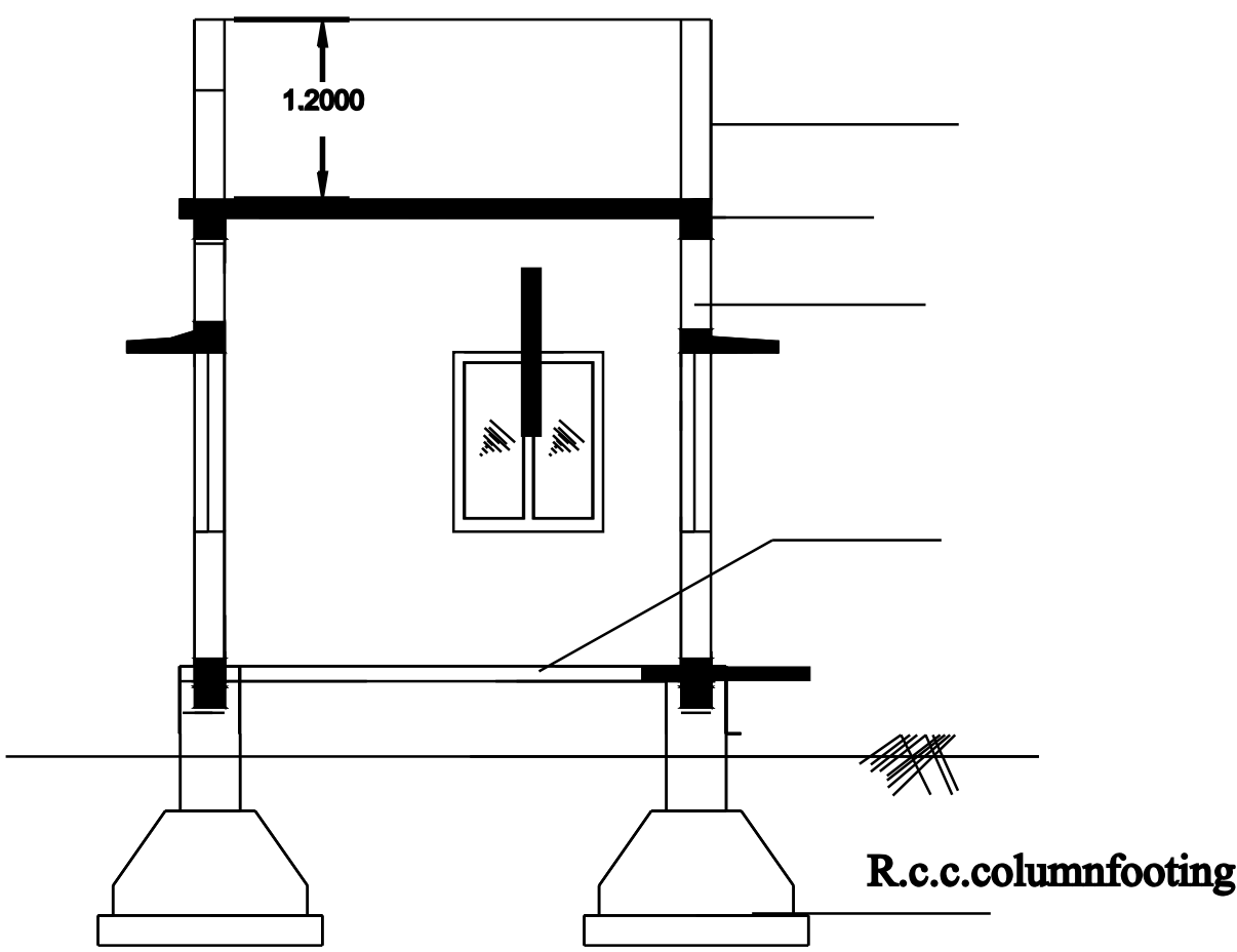
SECTION-AA
