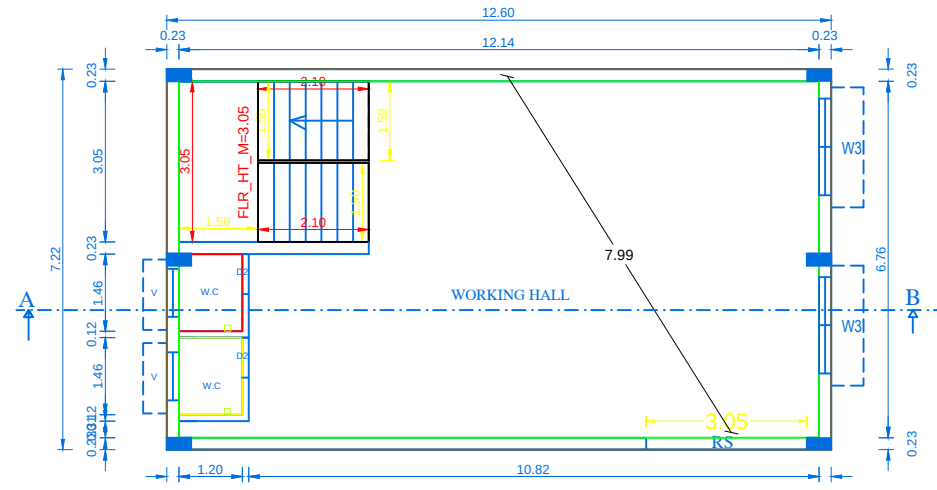
GROUND FLOOR PLAN (BLOCK-2)
