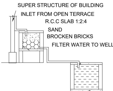
DETAILS OF FILTER BED & WELL
