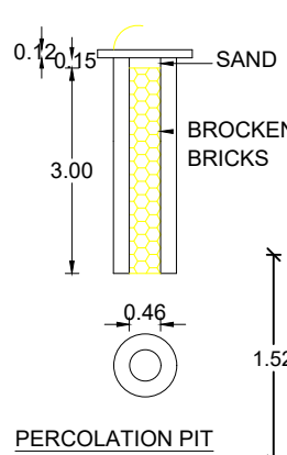
PERCOLATION PIT
