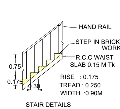
STAIR DETAILS
