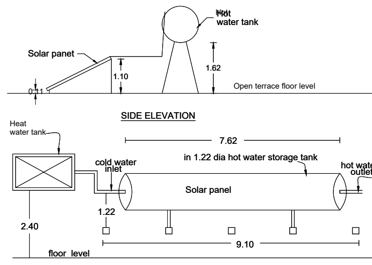
SOLAR WATER HEATER PLANT
