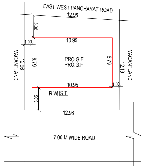
SITE PLAN
