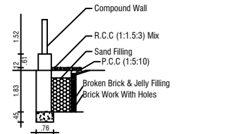
RAIN WATER HARVEST DETAILS
