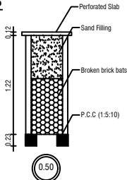
RAIN WATER COLLECTION WELL
