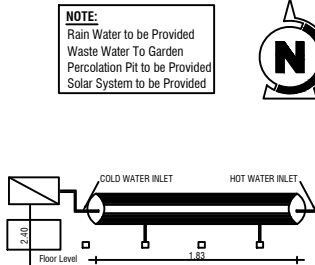
DETAILS OF SOLAR HOT WATER SYSTEM
