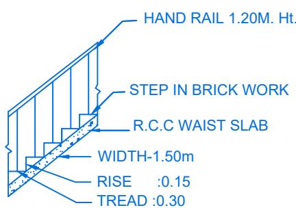
STAIR DETAIL
