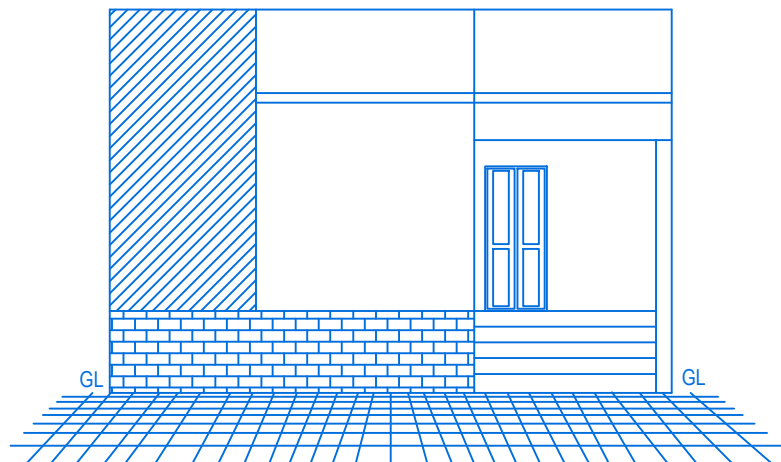
FRONT ELEVATION
