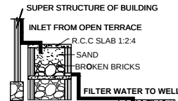
RAINWATER HARVESTING
