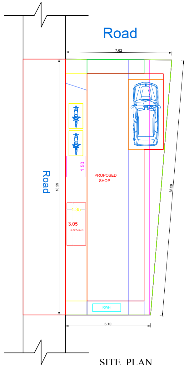
SITE PLAN
