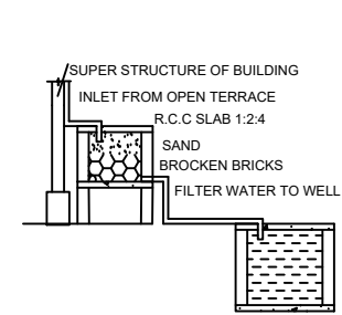
RAINWATER HARVESTING
