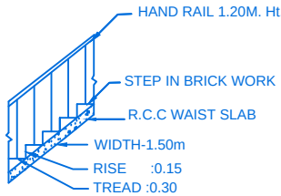
STAIR DETAIL
