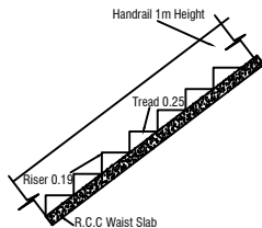
STAIR DETAILS
