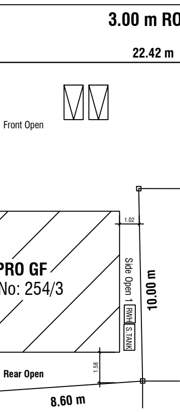
SITE PLAN (1:100)
