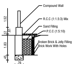
RAIN WATER HARVEST DETAILS
