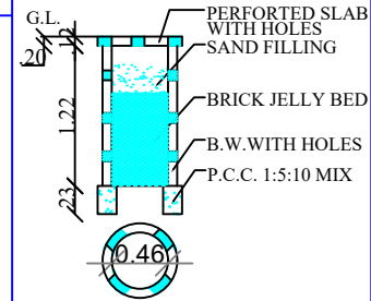
RAIN WATER HARVEST
