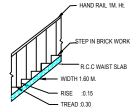
STAIR DETAIL
