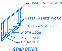
STAIR DETAIL
