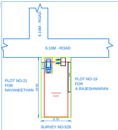
LOCATION PLAN Scale 1:400
