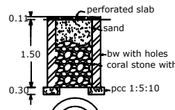
Percolation pit
