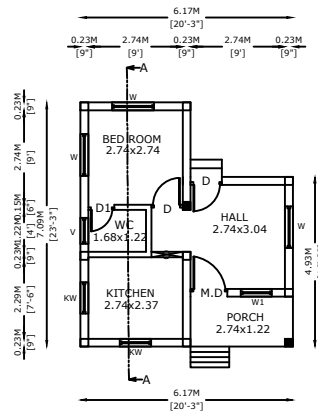
PRO.GROUND FLOOR
