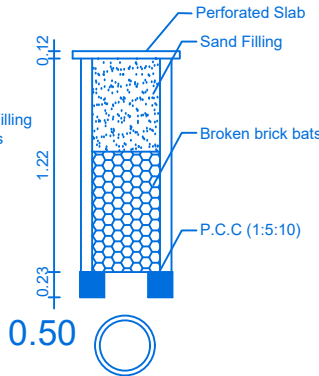
RAIN WATER COLLECTION WELL
