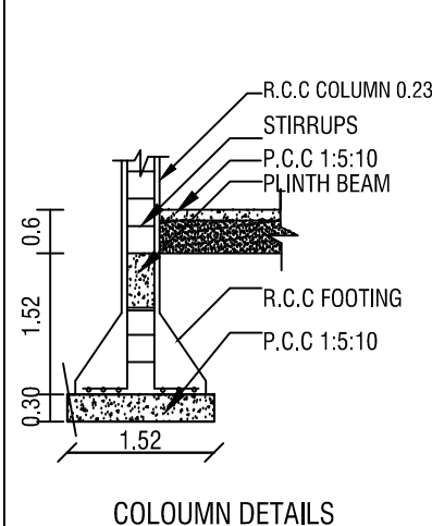
Column Details
