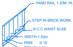
STAIR DETAIL
