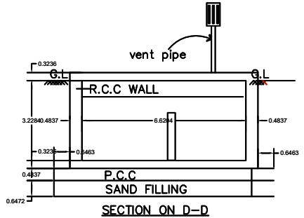
SECTION ON D-D
