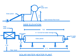
SOLAR WATER HEATER PLANT
