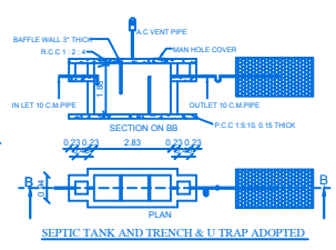
SEPTIC TANK AND TRENCH & U TRAP ADOPTED
