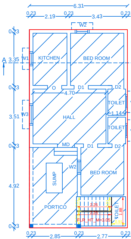
EXG.GROUND FLOOR PLAN
