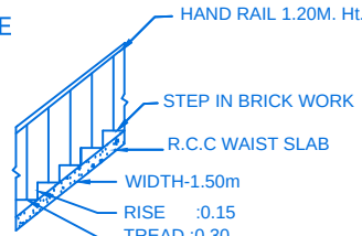
STAIR DETAIL
