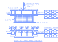
SECTION-TANK AND TRENCH
