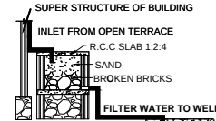
RAINWATER HARVESTING
