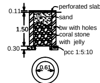
percolation pit
