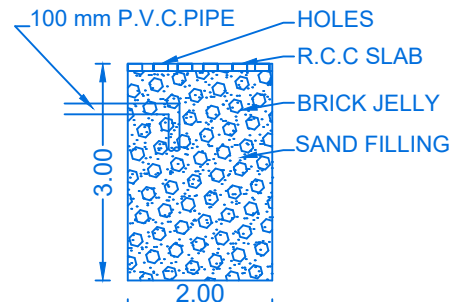
SECTION OF RAIN WATER COLLECTING TANK
