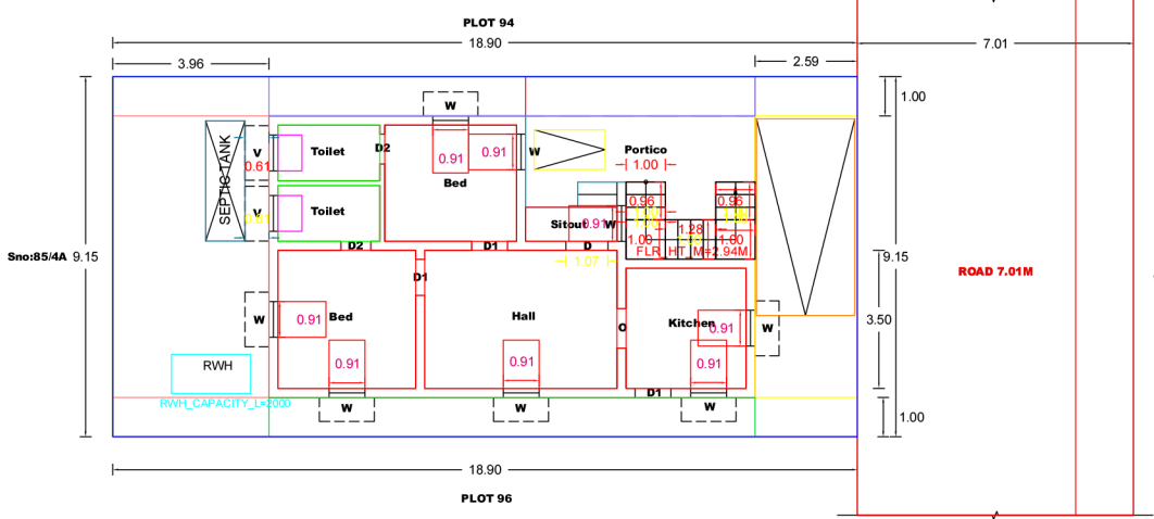
SITE PLAN FOR THE PROPOSAL
