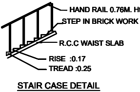
STAIR CASE DETAIL
