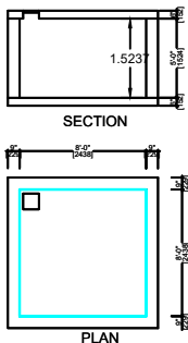
DETAILS OF COLLECTION SUMP FOR RAIN WATER HARVESTING OF ROOF TOP RAIN WATER RWH_CAPACITY_L=5000LTRS
