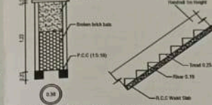
RAIN WATER COLLECTION WELL
