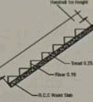
STAIR DETAILS
