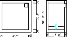
DETAILS OF COLLECTION SLUMP FOR RAIN WATER HARVESTING OF ROOF TOP RAINWATER RWH CAPACITY - L=5000LTS
