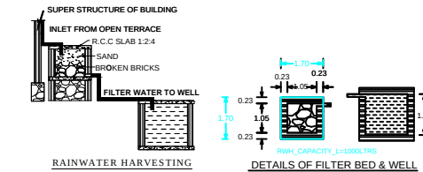
RAINWATER HARVESTING
