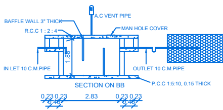
SEPTIC TANK AND TRENCH & U TRAP ADOPTED
