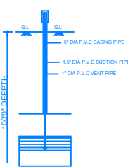
BORE WELL
