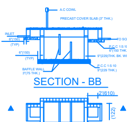
PLAN OF SEPTIC TANK
