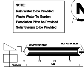
DETAILS OF SOLAR HOT WATER SYSTEM
