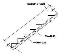
STAIR DETAILS
