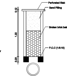
RAIN WATER COLLECTION WELL
