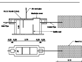
SEPTIC TANK & TRENCH
