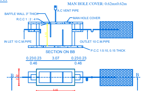
SEPTIC TANK AND TRENCH & U TRAP ADOPTED
