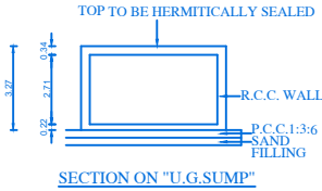
SECTION ON "U.G.SUMP"
