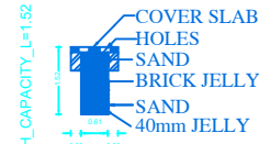
SECTION OF RAIN WATER COLLECTION TANK
