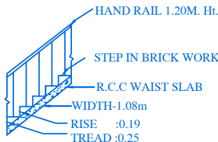
STAIR DETAIL
