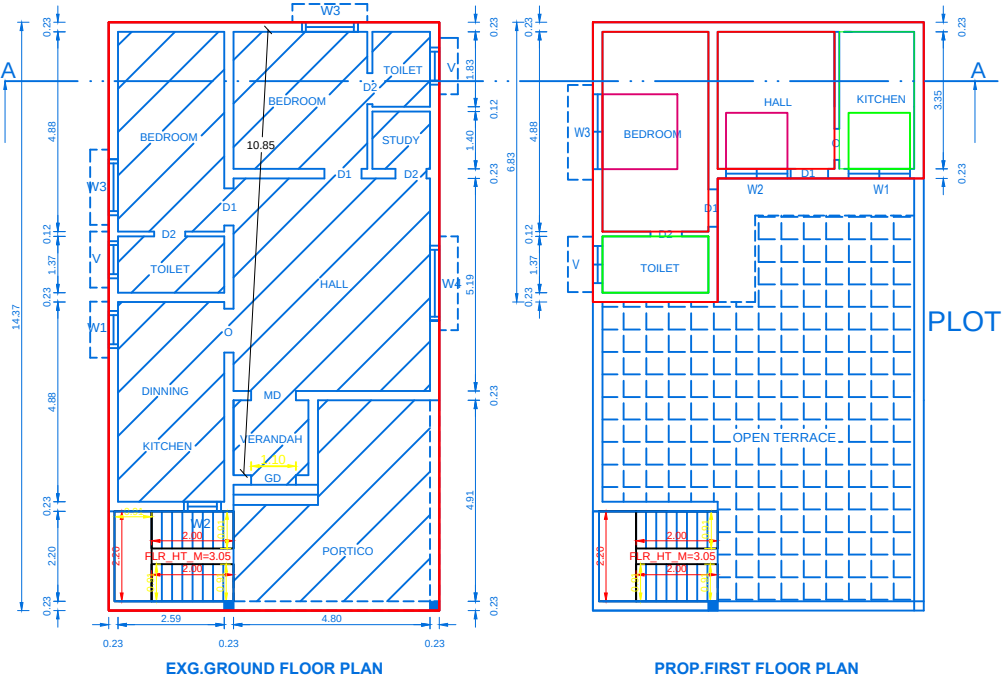
EXG.GROUND FLOOR PLAN
