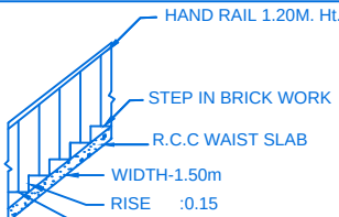
STAIR DETAIL
