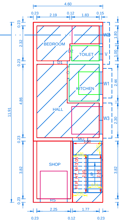
EXG & PROP.FIRST FLOOR PLAN
