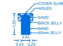
SECTION OF RAIN WATER COLLECTION TANK
