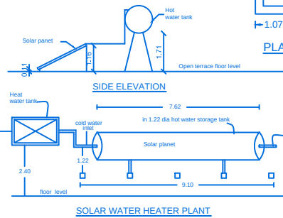
SOLAR WATER HEATER PLANT
