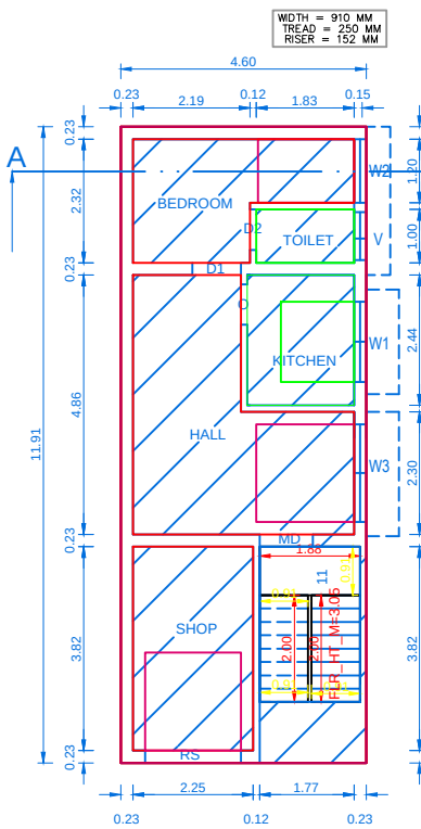
EXG.GROUND FLOOR PLAN
