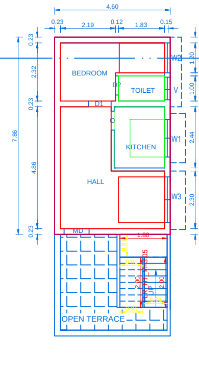
PROP.SECOND FLOOR PLAN
