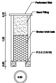
RAIN WATER COLLECTION WELL
