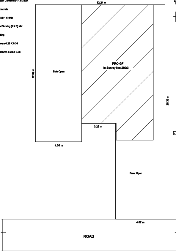
SITE PLAN (1:100)
