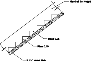
STAIR DETAILS
