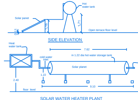
SOLAR WATER HEATER PLANT
