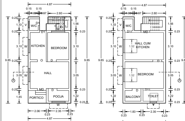
EXG.GROUND FLOOR PLAN
