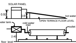
Details of solar water heating system
