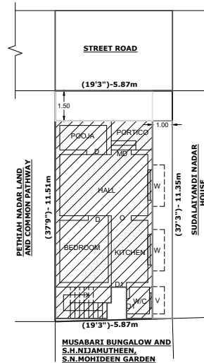
SITE PLAN (SCALE :- 1:100 )
