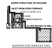
RAINWATER HARVESTING
