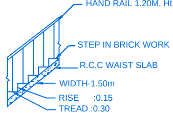
STAIR DETAIL
