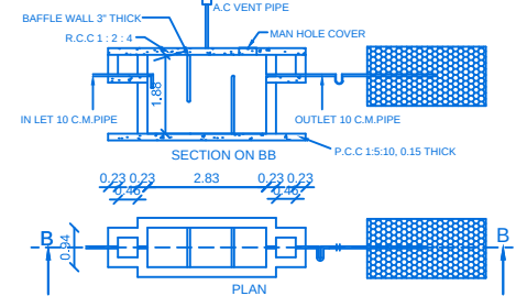
SEPTIC TANK AND TRENCH & U TRAP ADOPTED
