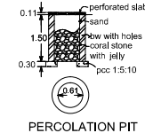
PERCOLATION PIT
