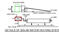
DETAILS OF SOLAR WATER HEATING SYSTEM
