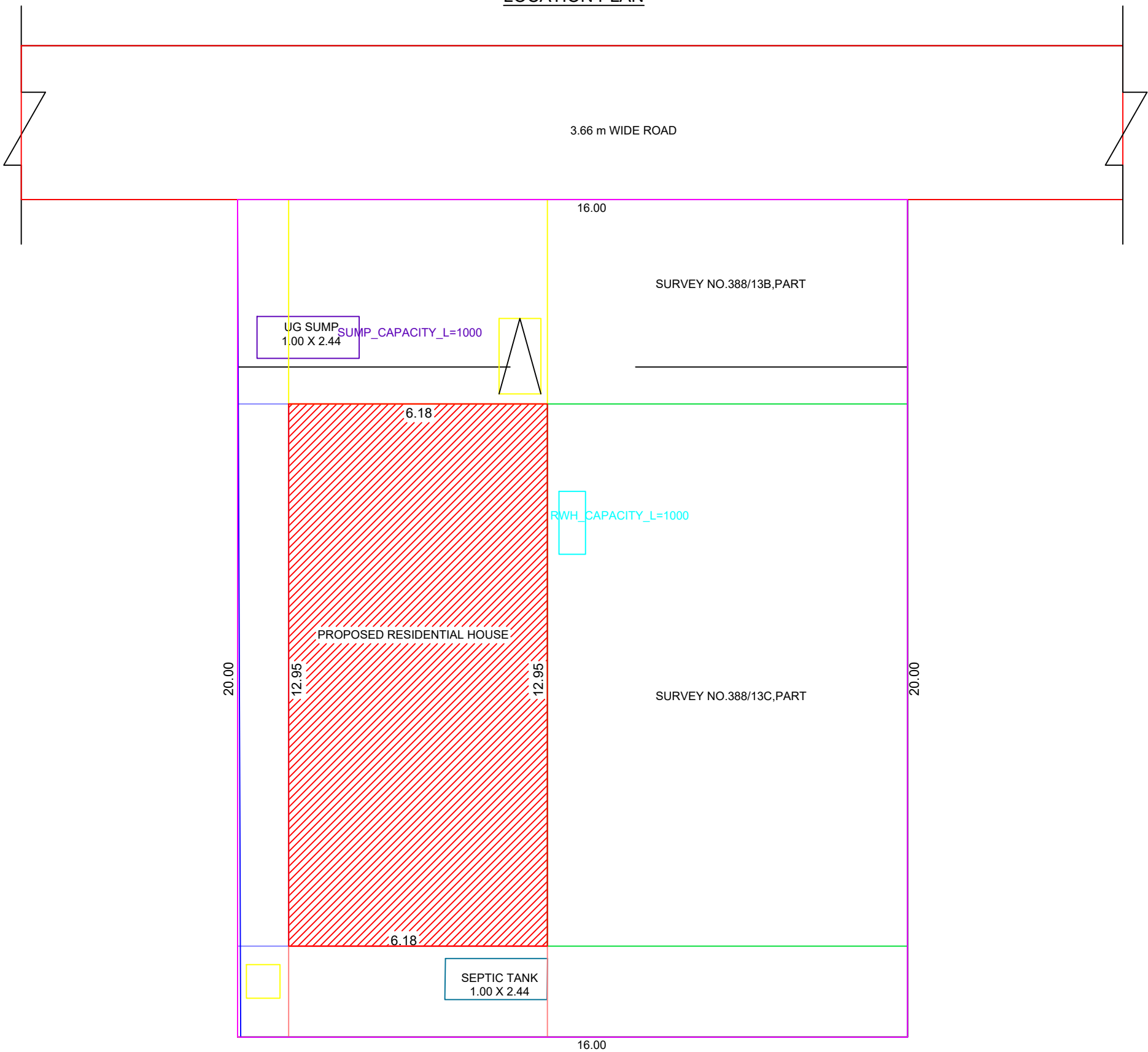
LOCATION PLAN
