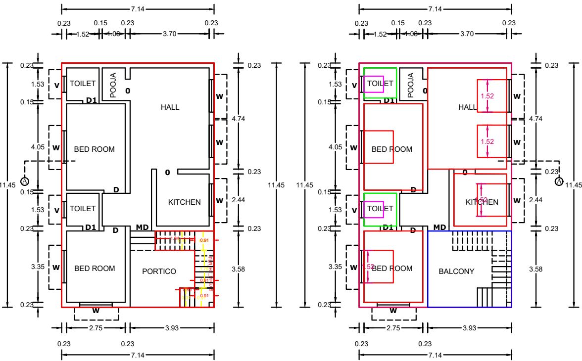
APPROVED GROUND FLOOR PLAN
