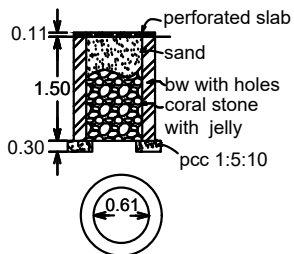
percolation pit
