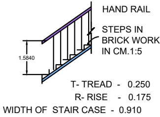
DETAILS OF STAIRCASE
