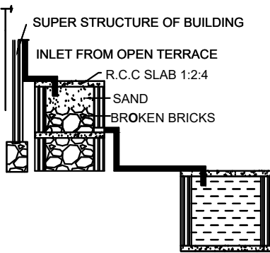
RAINWATER HARVESTING
