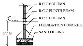
COLUMN DETAILS
