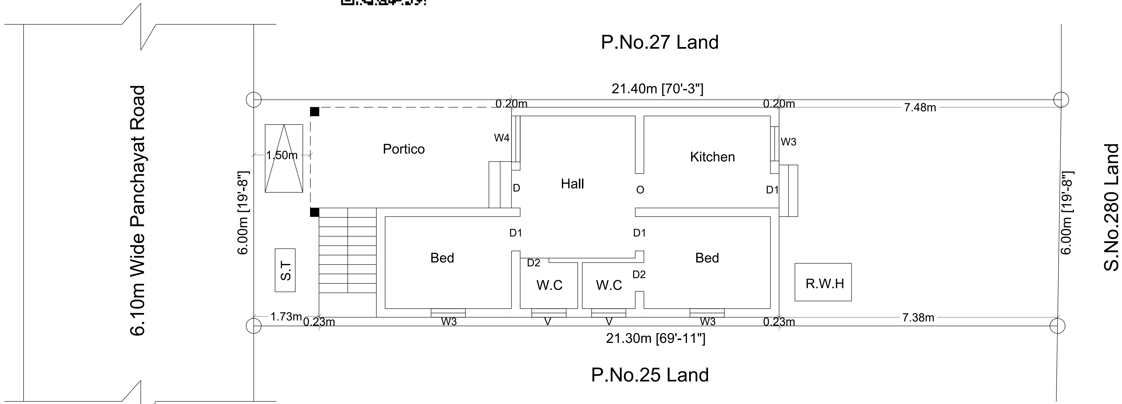
SITE PLAN
