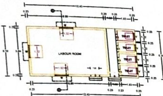
LABOUR ROOM PLAN
